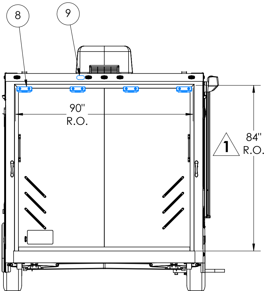
EXTERIOR REAR VIEW
